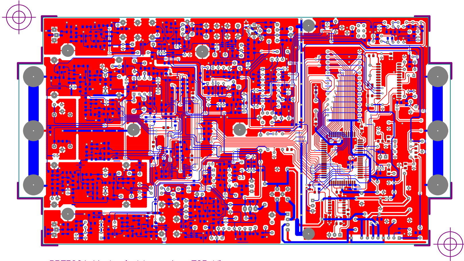
RPT300A Mechanical Layer 1 TOP View
